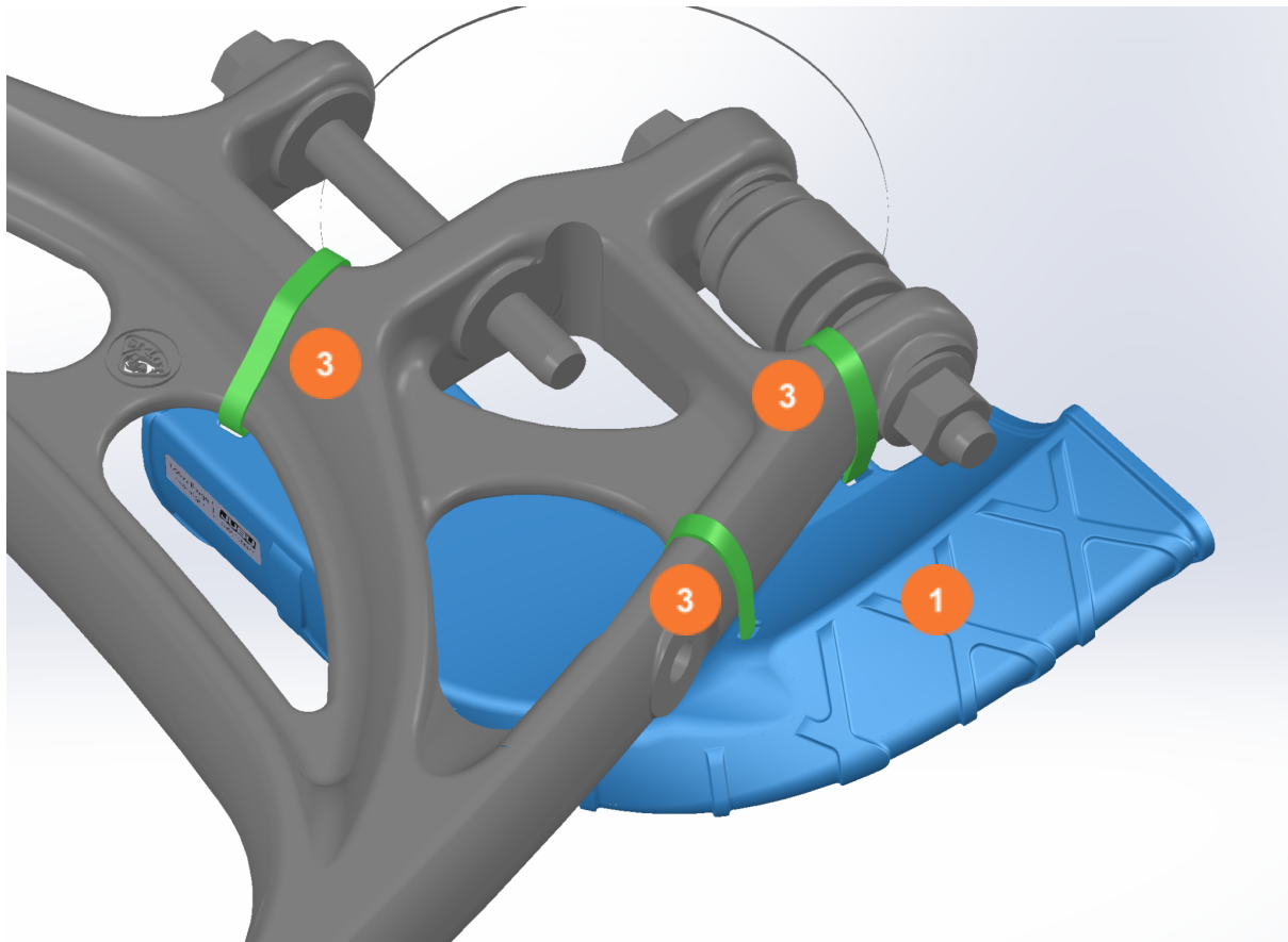
Fig. 2: Correct assembly and placement of the cable ties (rear right) (I)
