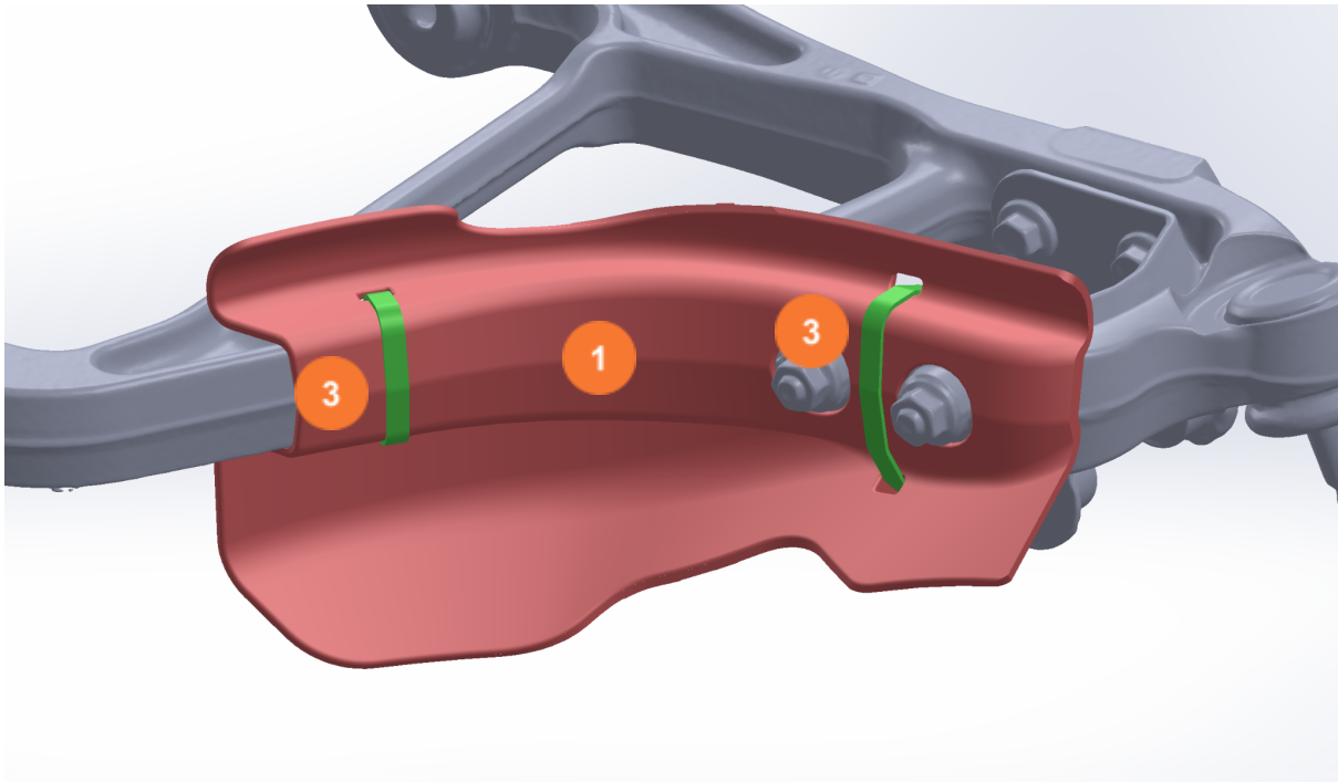
Fig. 2: Correct assembly and placement of the cable ties (front left) (I)
