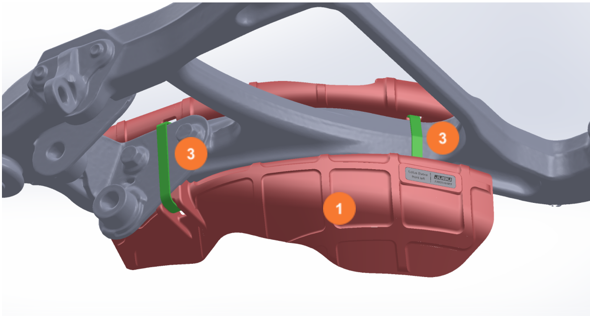
Fig. 3: Correct assembly and placement of the cable ties (front left) (II)
