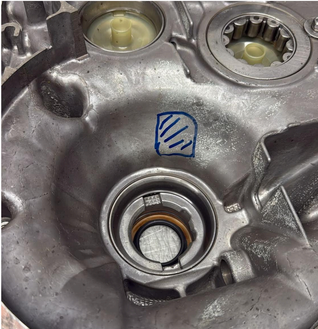
Fig 2: Machine the marked area if necessary
