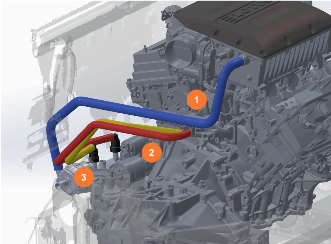
Fig 3: Connect the gearbox oil heat exchanger to the engine cooling circuit.(I)
