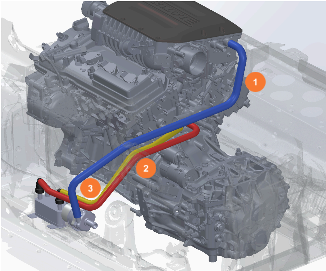
Fig 4: Connect the gearbox oil heat exchanger to the engine (II)
